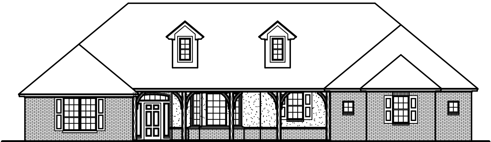
ELEVATION C
